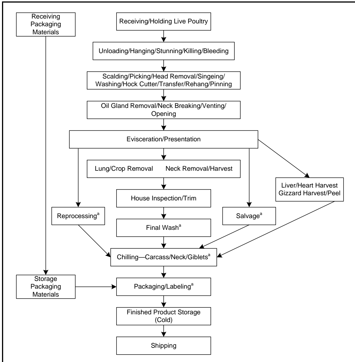
Figure 2-1. Process Flow Diagram: Young Chicken Slaughter
