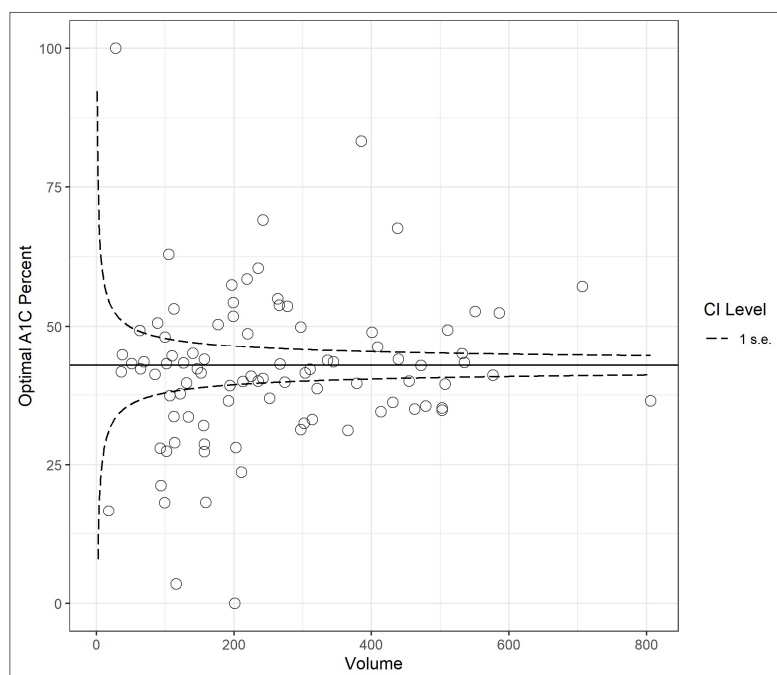
Figure 3. Example Funnel Plot of Optimal A1C Values for Patients 13-18 Years of Age on Private Insurance With Type 1 Diabetes and Patient Volume With 1 Standard Error Lines Used for Point Boundaries
