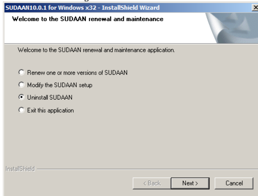
Figure 1.5 Uninstall SUDAAN
